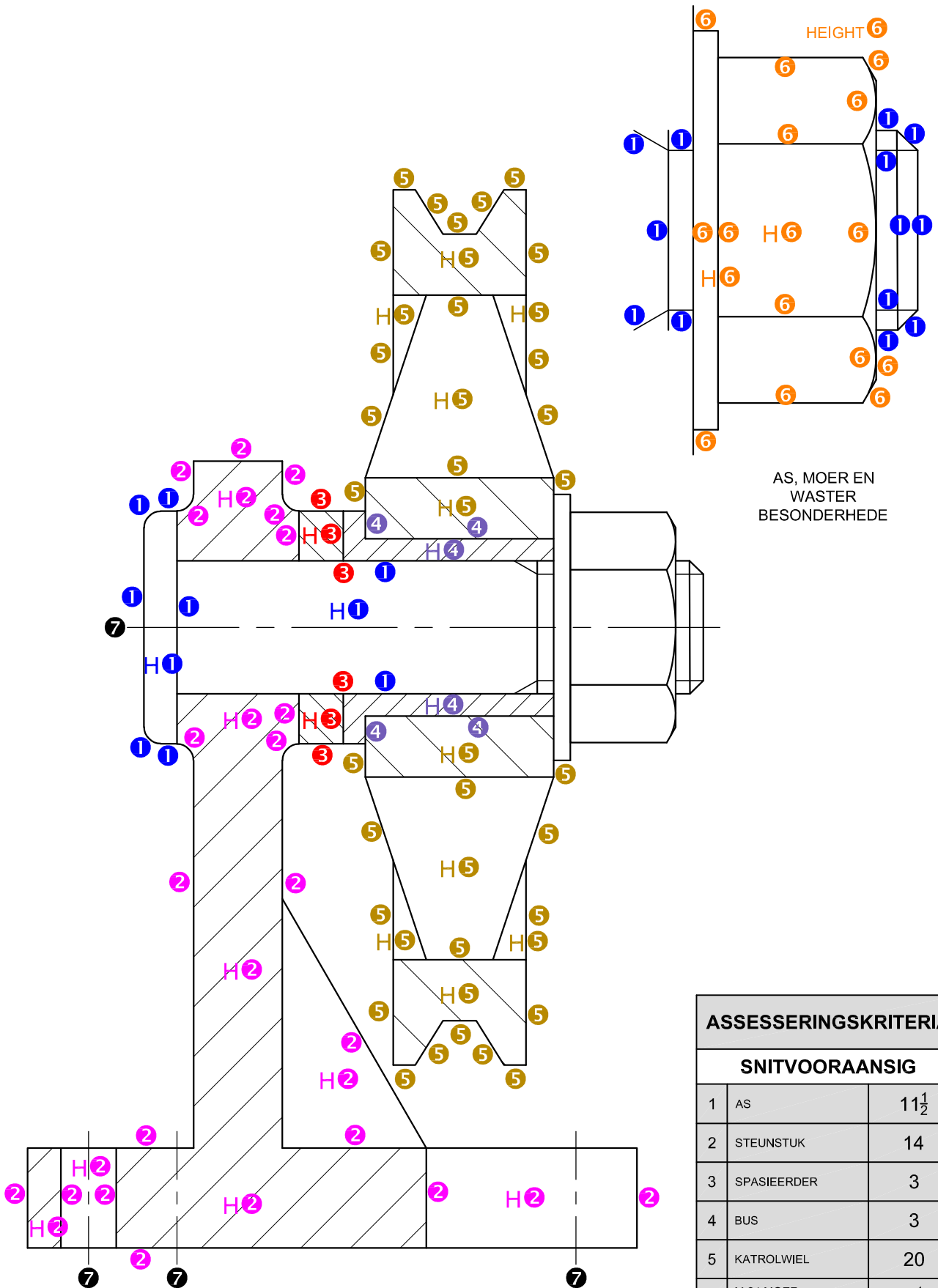
SECTION AA ✓
